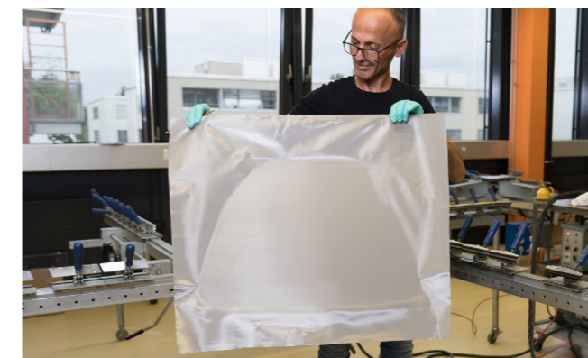
For additional protection, we bond the mesh to the filter frames.
